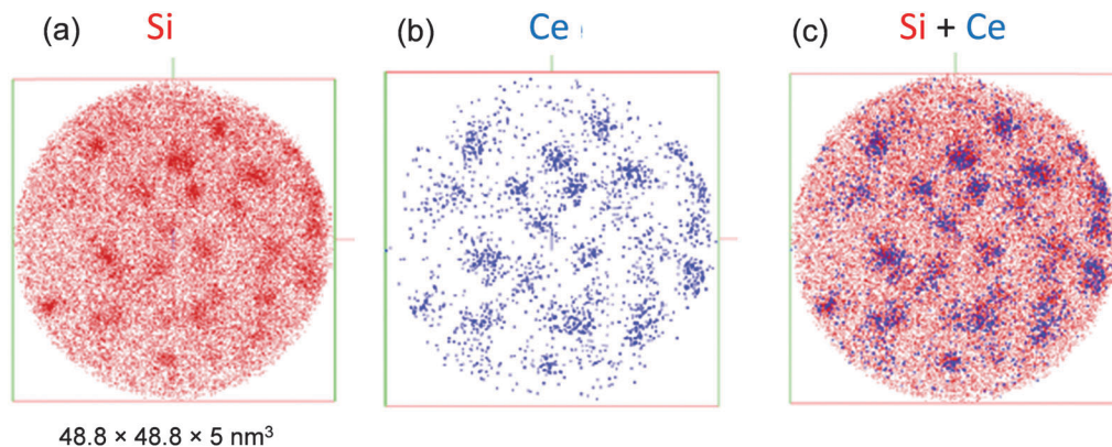
Fig. 4 Atom probe tomography analysis of the 3% Ce-doped \text{SiO}_{1.5} thin film annealed at 900\text{ }^\circ\text{C} . (a) Plane view of a 5\text{ nm} thick slice taken from the reconstructed volume. The Si atoms are shown as red dots, providing evidence of the presence of Si-rich clusters, (b) analogous plane view showing Ce atoms as blue dots, evidencing the presence of Ce-rich clusters, (c) superposition of the maps shown in (a) and (b) demonstrating that both Si- and Ce-rich clusters have the same locations. All the views have the size of 48.8 \times 48.8 \times 5\text{ nm}^3 .
