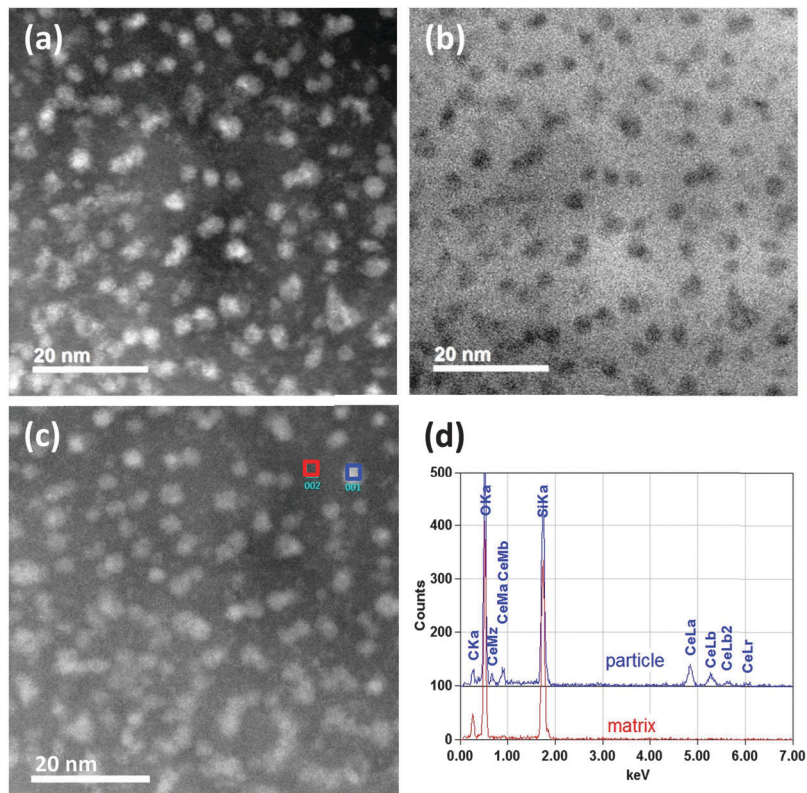
Fig. 3 HAADF image of a 3% Ce-doped \text{SiO}_{1.5} thin film annealed at 900\text{ }^\circ\text{C} showing the presence of Ce-rich clusters (a) and the corresponding bright field image (b). HAADF image (c) showing the areas (red square for the matrix and blue square for a particle) used for the EDS analysis (d)
