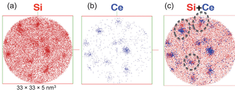
Fig. 6 Atom probe tomography analysis of the 3% Ce-doped \text{SiO}_{1.5} thin film annealed at 980 °C. (a) Plane view of a 5 nm thick slice taken from the reconstructed volume. The Si atoms are shown as red dots, providing evidence of the presence of Si-rich clusters, (b) analogous plane view showing Ce atoms as blue dots, evidencing the presence of Ce-rich clusters, (c) superposition of the maps shown in (a) and (b) demonstrating that both Si- and Ce-rich clusters no longer have the same locations (also indicated by dashed circles). All the views have the size of 33 \times 33 \times 5 \text{ nm}^3 .
