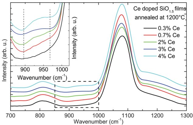
Fig. 8 FTIR spectra of Ce-doped \text{SiO}_{1.5} thin films annealed at 1200 °C. The Ce content is varied between 0.3% and 4%. All spectra are vertically offset for clarity. The dashed area is enlarged in the inset. The vertical dashed lines in the inset indicate the wavenumber range in which features corresponding to the formation of a cerium silicate are expected.
