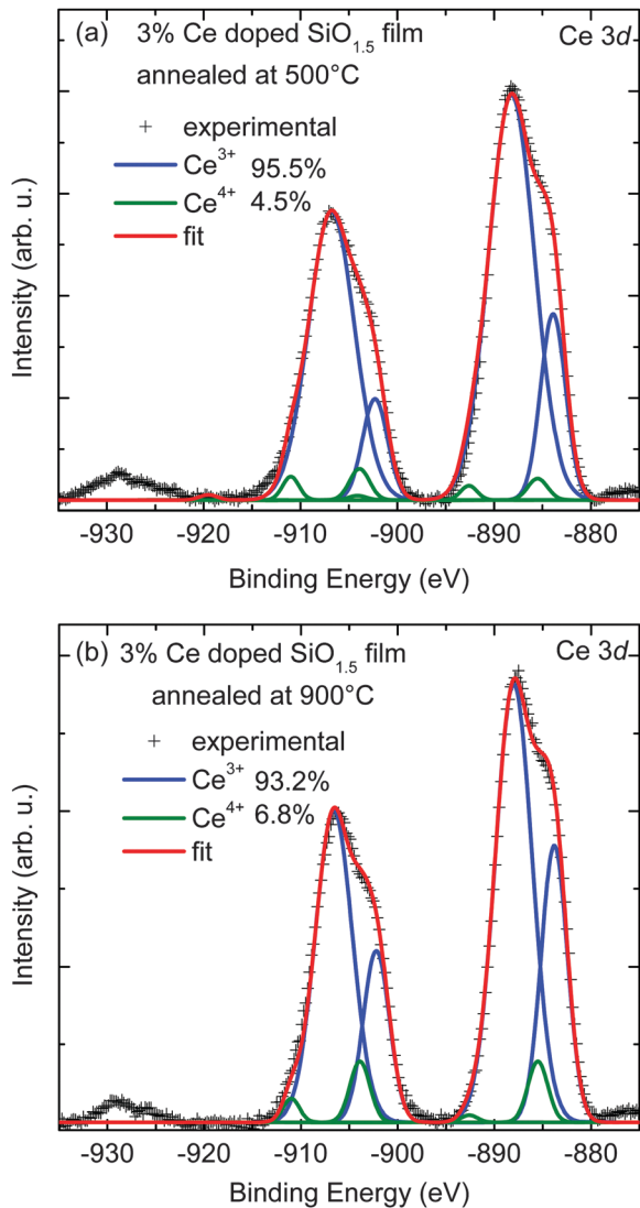
Fig. 2 X-ray photoelectron spectra of the Ce 3d core level measured on a 3% Ce-doped \text{SiO}_{1.5} thin film after annealing at 500 °C (a) and 900 °C (b). The result of the fit (solid lines) is superimposed on the experimental data (crosses).
