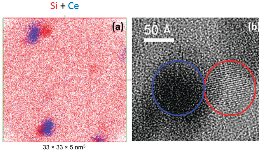
Fig. 7 Atom probe tomography analysis of the 3% Ce-doped \text{SiO}_{1.5} thin film annealed at 1100 °C. (a) Plane view ( 33 \times 33 \times 5 \text{ nm}^3 ) of a 5 nm thick slice taken from the reconstructed volume showing both Si atoms (red dots) and Ce atoms (blue dots). The phase separation between pure Si nanocrystals and Ce-rich clusters is evident. (b) High resolution cross sectional TEM image showing the presence of a pure Si nanocrystal (circled in red) in the immediate vicinity of a Ce-rich cluster (circled in blue).
