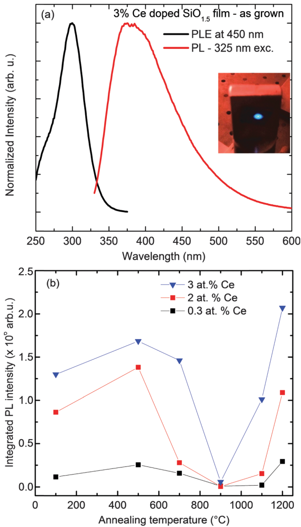
Fig. 1 (a) Steady state PL spectrum of a 3% Ce-doped \text{SiO}_{1.5} thin film measured at room temperature (red solid line). The corresponding PLE spectrum is shown as a black solid line. The inset shows a photograph of the sample showing the blue luminescence visible with the naked eyes. (b) Integrated Ce-related PL intensity as a function of annealing temperature for three different Ce contents.
