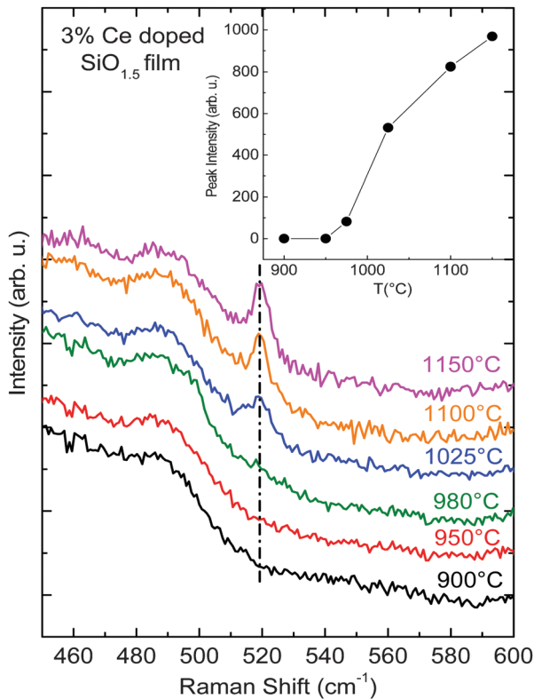
Fig. 5 Raman spectra measured on a 3% Ce-doped \text{SiO}_{1.5} thin film after annealing at various temperatures between 900 °C and 1150 °C. All spectra are vertically offset for clarity. The vertical dashed-dotted line indicates the position of the crystalline Si–TO peak at 520 \text{cm}^{-1} . The inset shows the evolution of the integrated Raman peak intensity at 520 \text{cm}^{-1} as a function of annealing temperature.
