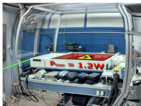
Figure 3: Augmented Reality application example on a dye laser. Visualization of invisible beam, delimitation of dangerous area, display of laser power during adjustments...
