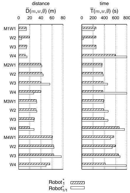
Fig. 16 Mission Performance without Injected Faults and with No Plan Repair
