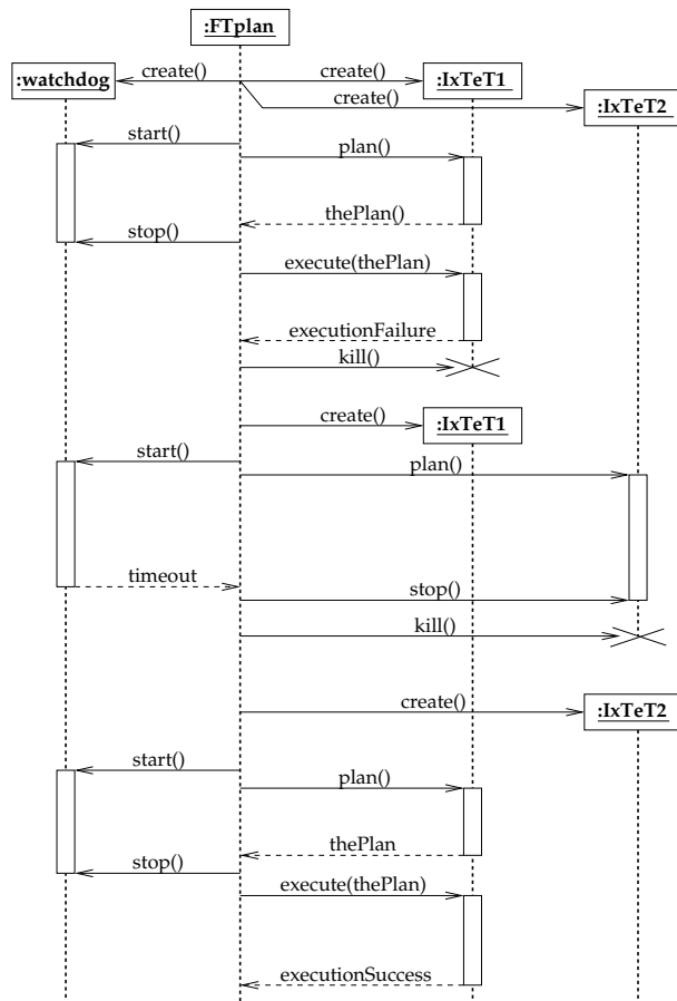
Fig. 6 A fault tolerance scenario with the sequential planning policy
