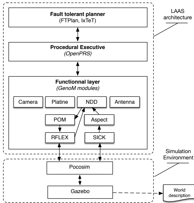
Fig. 7 Simulation environment
