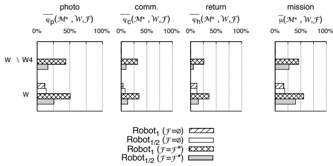
Fig. 20 Impact of planner redundancy in presence of faults
