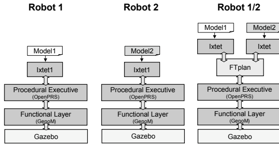
Fig. 12 Experimental Systems: Robot_1 , Robot_2 and Robot_{1/2}
