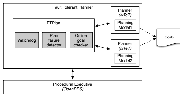
Fig. 5 Fault tolerant planner
