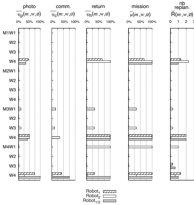
Fig. 13 Mission Undependability and Replannings without Injected Faults
