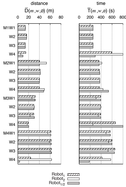
Fig. 14 Mission Performance without Injected Faults
