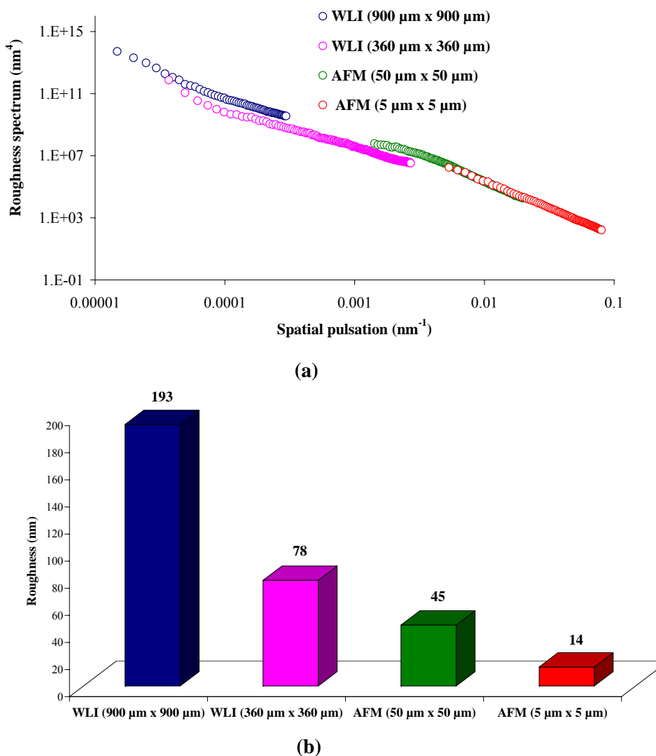
Figure 1. Roughness spectrum (a) and evolution of the roughness (b) for the 100 kDa flat sheet membrane by White Light Interferometry (WLI) and Atomic Force Microscopy (AFM).
