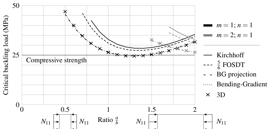
Fig. 5: Buckling load according to plate ratio \frac{a}{b} for 5ply-CLT with slenderness \frac{b}{h} = 20
