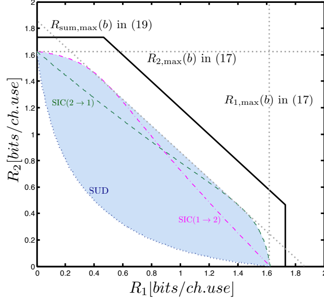
Figure 3: Projection of the set \mathcal{N}_{\text{SUD}}(b) (dotted line) and \mathcal{N}_{\text{SIC}(i \rightarrow j)}(b) (dashed lines) over the R_1 - R_2 plane for b = 0.7B_{\max} > 1 + \text{SNR}_{21} + \text{SNR}_{22} . The information capacity region without energy transmission constraints (region inside solid lines) is plotted for \text{SNR}_{11} = \text{SNR}_{12} = \text{SNR}_{21} = \text{SNR}_{22} = 10 (Note that B_{\max} \triangleq 1 + \text{SNR}_{21} + \text{SNR}_{22} + 2\sqrt{\text{SNR}_{21}\text{SNR}_{22}} ). The blue region is the convex hull of \mathcal{N}_{\text{SUD}}(b) \cup \mathcal{N}_{\text{SIC}(1 \rightarrow 2)}(b) \cup \mathcal{N}_{\text{SIC}(2 \rightarrow 1)}(b) .
