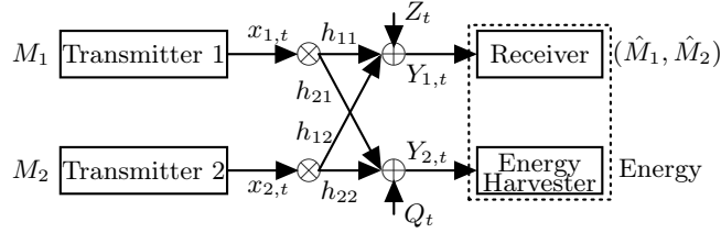
Figure 1: Two-user memoryless Gaussian MAC with energy harvester.
