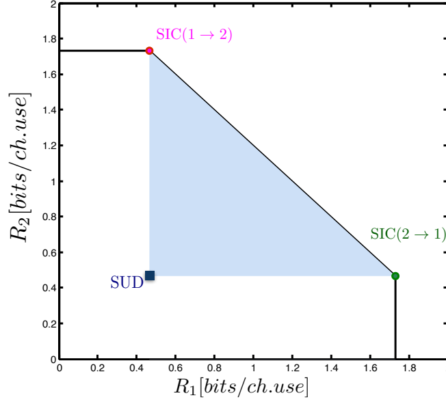
Figure 2: Projection of the set \mathcal{N}_{\text{SUD}}(b) (square point) and \mathcal{N}_{\text{SIC}(i \rightarrow j)}(b) (round points) over the R_1 - R_2 plane for b \leq 1 + \text{SNR}_{21} + \text{SNR}_{22} . The information capacity region is also plotted as a reference (white region inside solid lines) for \text{SNR}_{11} = \text{SNR}_{12} = \text{SNR}_{21} = \text{SNR}_{22} = 10 . Note that the information capacity region with and without energy transmission rate constraint are identical in this case. The blue region is the convex hull of \mathcal{N}_{\text{SUD}}(b) \cup \mathcal{N}_{\text{SIC}(1 \rightarrow 2)}(b) \cup \mathcal{N}_{\text{SIC}(2 \rightarrow 1)}(b) .
