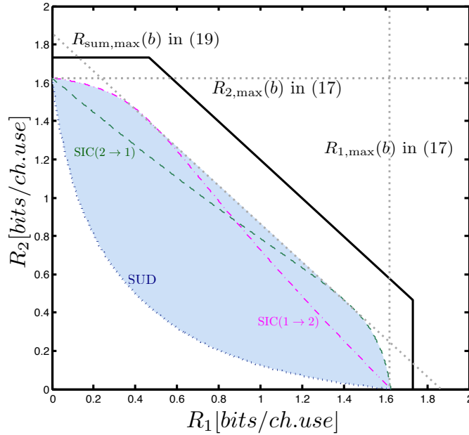
Figure 3: Projection of the set \mathcal{N}_{\text{SUD}}(b) (dotted line) and \mathcal{N}_{\text{SIC}(i \rightarrow j)}(b) (dashed lines) over the R_1 - R_2 plane for b = 0.7B_{\max} > 1 + \text{SNR}_{21} + \text{SNR}_{22} . The information capacity region without energy transmission constraints (region inside solid lines) is plotted for \text{SNR}_{11} = \text{SNR}_{12} = \text{SNR}_{21} = \text{SNR}_{22} = 10 (Note that B_{\max} \triangleq 1 + \text{SNR}_{21} + \text{SNR}_{22} + 2\sqrt{\text{SNR}_{21}\text{SNR}_{22}} ). The blue region is the convex hull of \mathcal{N}_{\text{SUD}}(b) \cup \mathcal{N}_{\text{SIC}(1 \rightarrow 2)}(b) \cup \mathcal{N}_{\text{SIC}(2 \rightarrow 1)}(b) .
