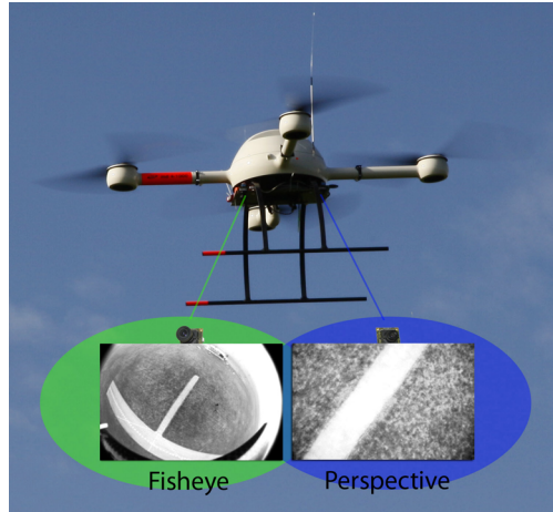
Figure 2: A perspective an fisheye stereo rig embedded on a UAV and their images.
