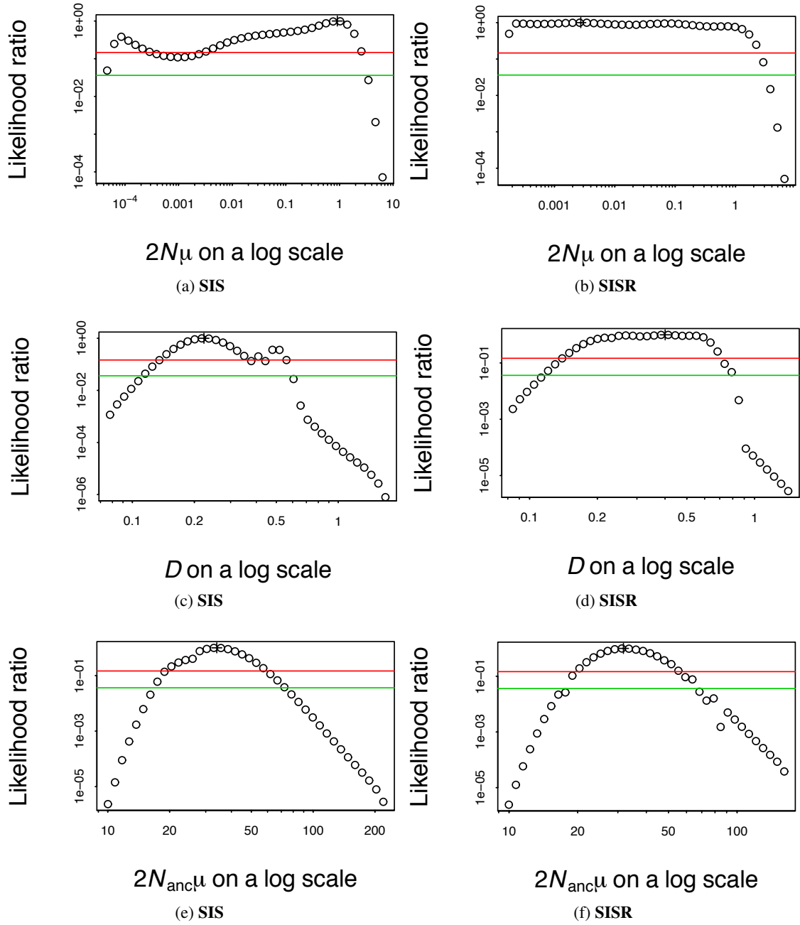
Figure 11: One-parameter profile likelihood ratios. (a) and (b) represent the likelihood profile function divided by its maximum value \theta \mapsto \hat{L}_\theta(\hat{D}_\theta, \hat{\theta}_{anc \theta}) / \hat{L}(\hat{\theta}, \hat{D}_\theta, \hat{\theta}_{anc \theta}) , (c) and (d) represent in the same way the profile likelihood ratio for D and (e) and (f) represent the profile likelihood ratio for \theta_{anc} , estimated respectively with SIS (left) or with SIRS (right). See Appendix. C for details on profile likelihood.
