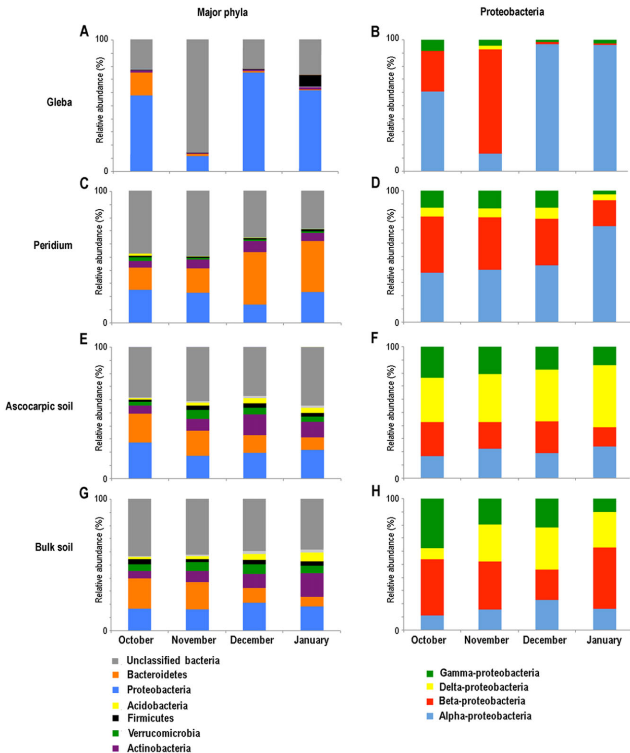
Fig. 3. Evolution of the relative distribution of the major phyla (A, C, E, G) and proteobacteria classes (B, D, F, H) in the different compartments considered (gleba, peridium, ascocarpic adhering soil and bulk soil) along truffle maturation (from October 2010 to January 2011).
