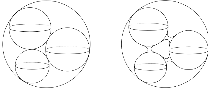
FIGURE 1. Left: a packing of three horospheres with three tangency points in the ball model of \mathbb{H}^3 . Right: a CMC-1 surface of genus one with three ends.
