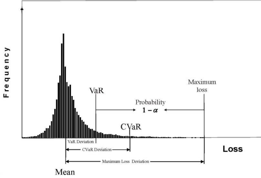
Figure 4: difference between VaR and CVaR
