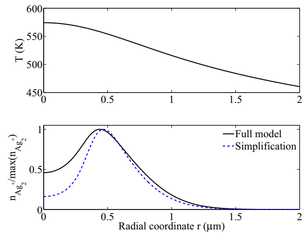
FIG. 4. (Top) Radial distribution of lattice temperature. (Bottom) Radial distribution of the silver cluster concentration n_{Ag_2^+} . Full model (black solid line) and simplified model (blue dashed line) predictions are provided. The input laser pulse energy is E_0 = 200 \text{ nJ} , number of pulses is N_p = 1000 . Dissociation function parameters are: S_0 = 80 , N = 6 .
