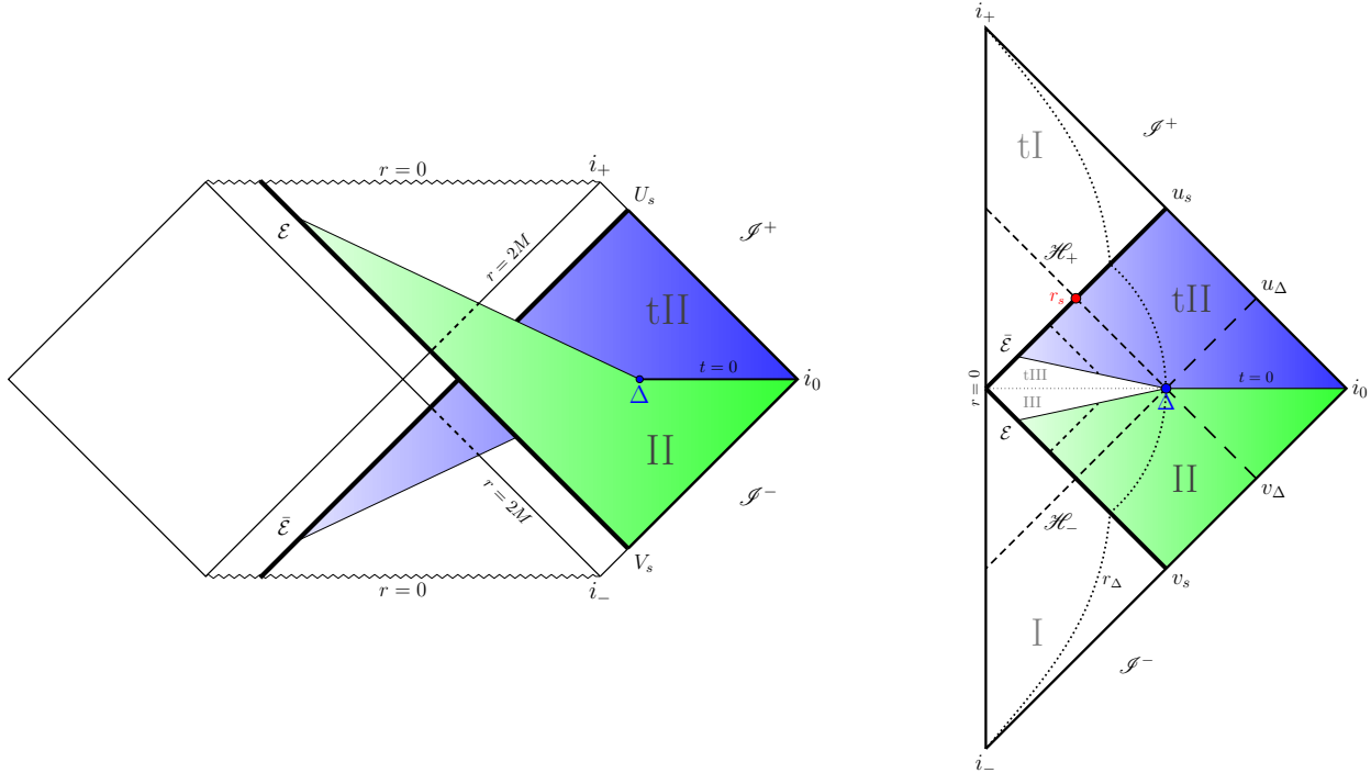
FIG. 1: Geometry of the black hole fireworks scenario. Left: Kruskal-Szekeres diagram, with the two interesting overlapping regions shaded with different colors. Right: The resulting completely time-symmetric Carter-Penrose diagram.
