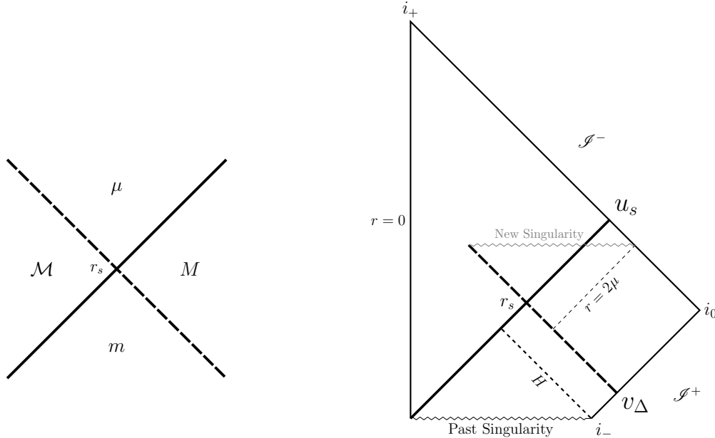
FIG. 3: Left: The Dray-'t Hooft geometry. Four Schwarzschild patches with different masses are glued together along null shells which intersect at a radius r_s . The condition for the geometries to be glued smoothly generates a relation between the four masses and r_s . Right: The death of a white hole. A white hole emits all its mass m along a massive null shell at the retarded time u_s . A small massive perturbation \nu is sent at the advanced time v_\Delta into the white hole geometry and interact with the outgoing shell at r = r_s . At the interaction point we have a Dray-'t Hooft geometry with m = m , \mathcal{M} = 0 , M = m + \nu . The last mass \mu is uniquely determined by the constraint which leads to eq. (23): \mu = r_s/(r_s - 2m)\nu . If r_s is lower than 2\mu , the emerging shell is captured in the future black hole horizon of the new geometry generated by the interaction and cannot escape to infinity. The white hole is dead recollapsing into a black hole.
