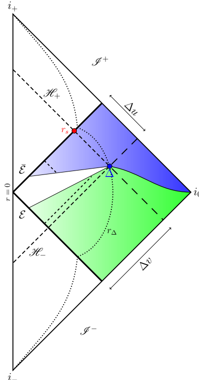
FIG. 2: Geometry of a asymmetric bouncing scenario. The parameter \Delta v \sim m^2 captures both the accumulation time for quantum gravitational effect outside the horizon and the lifetime of the hole. The parameter \Delta u , on the other hand, represents the lifetime of the white hole and it is forced by the arguments presented in the text to be of order m \log m .
