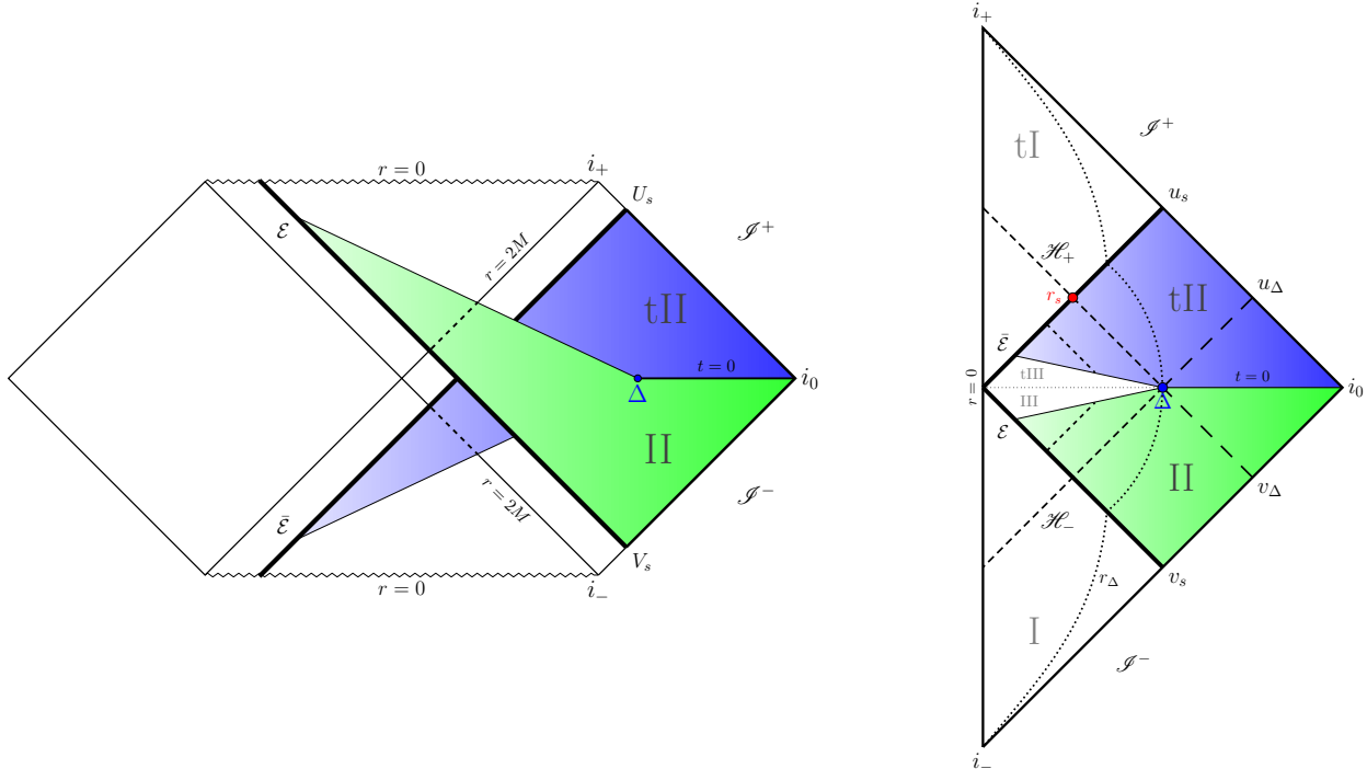
FIG. 1: Geometry of the black hole fireworks scenario. Left: Kruskal-Szekeres diagram, with the two interesting overlapping regions shaded with different colors. Right: The resulting completely time-symmetric Carter-Penrose diagram.
