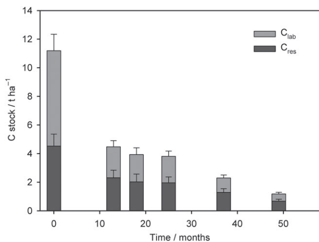
Figure 4 Stock of labile carbon pool ( C_{lab} ) and resistant carbon pool ( C_{res} ) of woody debris > 4 mm in the 0–30-cm layer. Values are means, error bars represent standard errors ( n = 14 at the beginning of the experiment, n = 18 at the 13th and 18th months, n = 72 at the 25th, 37th and 49th months). See Table 3 for the calculation of variables.
