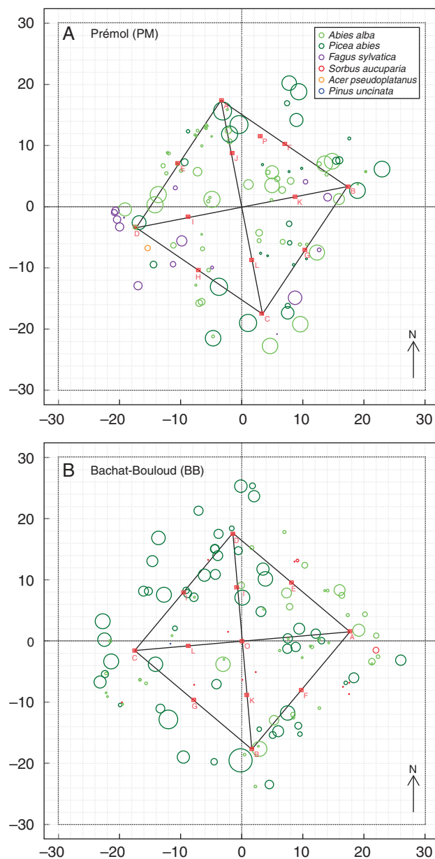
FIG. 1. Mapping of mini-monoliths (squares) and tree trunks of different species (circles of different colours) based on forest inventories in 2009 and 2010. x - and y -axes are distances in metres. The diameter of each tree trunk has been enlarged five times for easier viewing.
