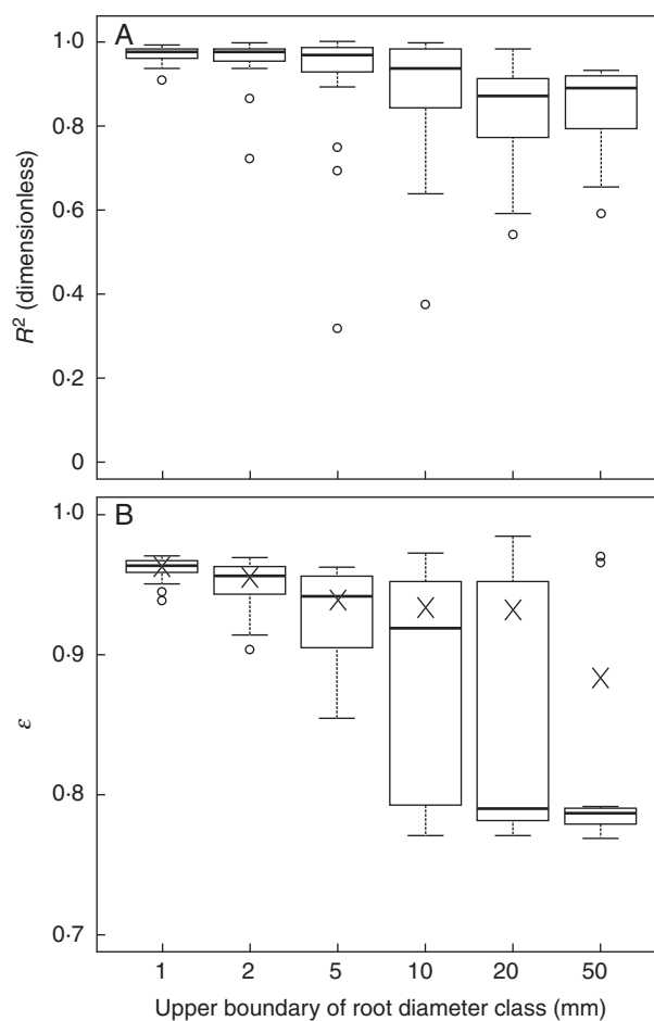
FIG. 8. Fit comparisons of the sub-models of vertical profile between different classes of root diameter. Boxplots in (A) and (B) show the quantiles of R^2 and \epsilon of the one-curve-per-replicate fits, respectively ( N_r = 24 ). In (B), crosses denote the value of \epsilon for the global fits to all the root data within one diameter class; hollow points denote outliers. \epsilon is the coefficient of the root profile shape. The closer \epsilon approaches 1, the more the roots tend to be less concentrated at the soil surface.
