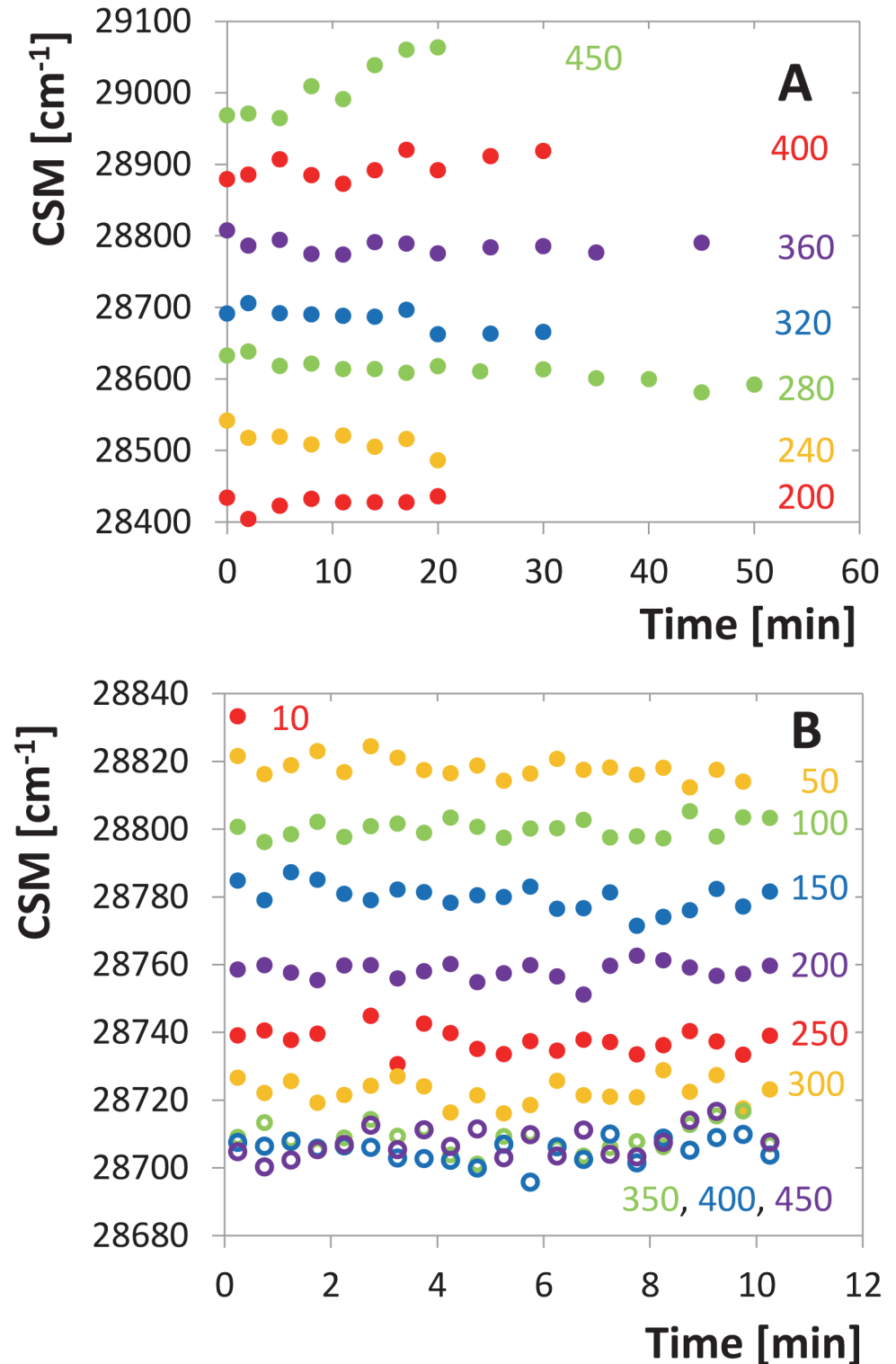
Fig 4. Time development of the tryptophan-fluorescence CSM. A. Time series for different pressures, each started with a new enzyme sample, concentration of 10 μM dimer. The individual curves are shifted up or down by artificially chosen constant for the sake of better orientation in the graph. B. Time series measured with the same sample of 2 μM concentration, pressure setting is facilitated by pressure jumps. The CSM scale is genuine for all the series.
