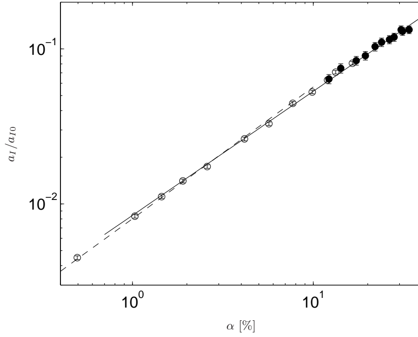
FIGURE 6. Interfacial area (Eq. 2.7) versus gas volume fraction: • this work; ○ from Colombet et al. (2011); -- equation 3.3; — equation 3.4.
