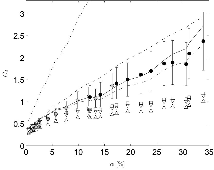
FIGURE 11. Experimental drag coefficient (Eq. 3.7) against gas volume fraction: \bullet method using a fixed focal lens; \circ method using a telecentric lens. Drag coefficient for a single bubble of same equivalent diameter rising at its terminal velocity (Eq. 3.8): \square Mendelson (1967); \nabla Comolet (1979); \triangle Dijkhuizen et al. (2010). Drag coefficient accounting for the collective effect of the bubbles: — Wallis (1961) (Eq. 3.9); -.- Ishii & Chawla (1979) (Eq. 3.10); \cdots Garnier et al. (2002) (Eq. 3.11); --- Roghair et al. (2011) (Eq. 3.12).
