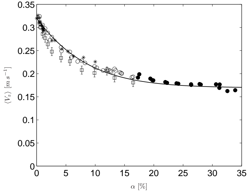
FIGURE 7. Average bubble velocity against the gas volume fraction. Dual-tip optical probe measurements from this work (●), Colombet et al. (2011) (○), Riboux et al. (2010) (*). Particle Tracking Velocimetry by image processing from Colombet et al. (2011) (□). — equation (3.5).
