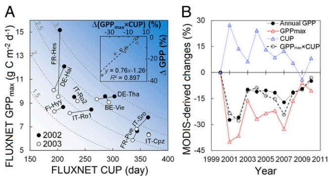
Fig. 2. Applications of the convergence of \alpha (the ratio between annual GPP and GPP_{max} \times CUP ) to explain GPP response to and recovery from disturbances. (A) Determination of the annual GPP reduction during the European heatwave in 2003 (12) by GPP_{max} and CUP. The dashed hyperbolic curves represent constant values (shown near the curves) of GPP_{max} \times CUP (kilograms C meter -2 year -1 ), and the darker background blue color means a larger GPP_{max} \times CUP . Inset shows the dependences of the relative changes in annual GPP ( \Delta GPP ; percentage) in 2003 from those in 2002 on the relative changes in GPP_{max} \times CUP [ \Delta(GPP_{max} \times CUP) ; percentage; black circles]. The ten sites are: BE-Vie (Vielsalm, Belgium), DE-Hai (Hainich, Germany), DE-Tha (Tharandt, Germany), Fi-Hyy (Hyytiälä, Finland), FR-Hes (Hesse Forest- Sarrebourg, France), FR-Pue (Puechabon, France), IT-Cpz (Castelporziano, Italy), IT-Ro1 and IT-Ro2 (Roccarespanpani, Italy), IT-Sro (San Rossore, Italy). Detailed information about each FLUXNET site can be found in SI Appendix, Fig. S9 and Table S1. (B) Contrasting dynamics of GPP_{max} and CUP after an extensive wildfire in the Black Hills National Forest in South Dakota. The data were extracted from a burned 0.1^\circ \times 0.1^\circ grid cell ( 43.85^\circ \text{ N} , 103.95^\circ \text{ W} ) (original data are plotted in SI Appendix, Fig. S2). The ratio \alpha was close to 0.62 during the 11-y span (SI Appendix, Fig. S10).
