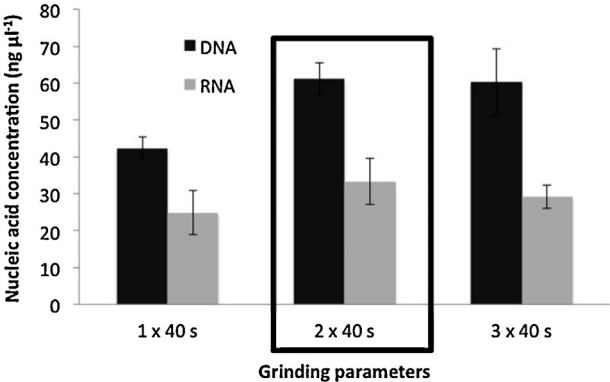
Fig. 3. Concentrations of nucleic acids extracted (DNA and RNA) in function of the number of 40-s grinding cycles at 6 m s -1 performed by the FastPrep™ instrument. Errors bars correspond to 95% confidence intervals (alpha 0.05, 3 replicates). The conditions chosen as standard are framed.
