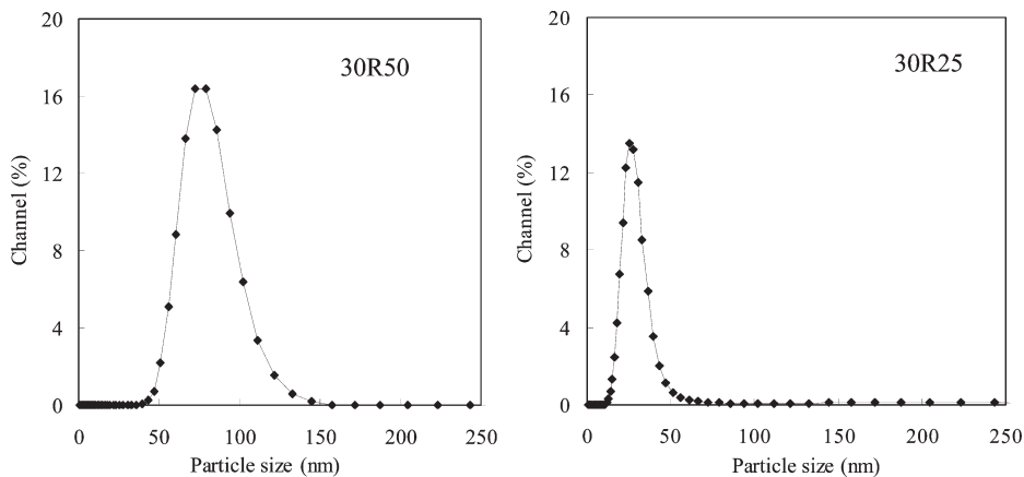
Figure 2. PSD of the Klebosol 30R50 and 30R25 suspensions measured by the Nanotrac.
