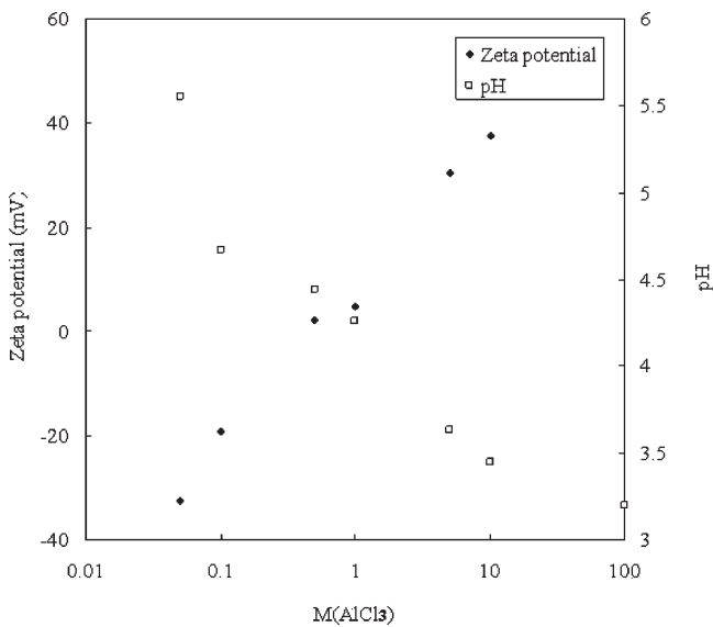
Figure 8. Zeta potential and pH profiles of the 30R50 (0.15%) at different concentrations of \text{AlCl}_3 (mmol·L -1 ).
