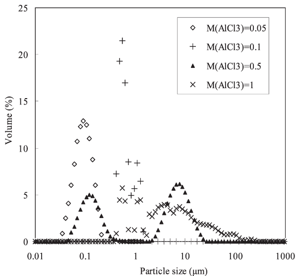
Figure 9. Particle size of the 30R50 (0.15%) with different concentrations of \text{AlCl}_3 (mmol·L -1 ) analyzed by Mastersizer 2000.
