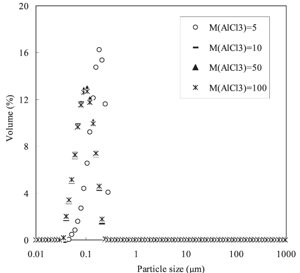
Figure 9. Particle size of the 30R50 (0.15%) with different concentrations of \text{AlCl}_3 (mmol·L -1 ) analyzed by Mastersizer 2000.
