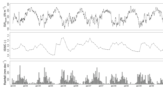
Fig. 3. Seasonal patterns in \text{SW}_{\text{down}} , index of soil water content (ISWC) and rainfall at Guyaflux over 2004–2009 (data from Bonal et al., 2008 and from this study).
