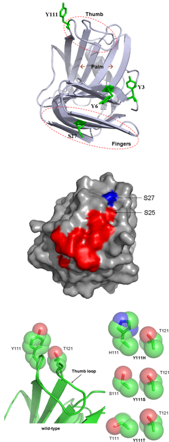
Figure 6 Localization of key mutations in the three-dimensional structure of Thermobacillus xylanilyticus xylanase (Tx-Xyn). (A) Positions of Y3, Y6, S27 and Y111 residues. (B) Potential secondary binding site determinants (red), including S27 (blue), mutated in this study. (C) Space-filling model showing the spatial occupation of side chains at positions 111 and 121 in Tx-Xyn and in the mutants Y111H, Y111S and Y111T. All figures were prepared using PyMol software [64].
