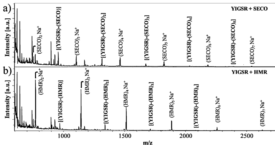
Fig. 6. MALDI-TOF mass spectra from VP-heteropolymerization of YIGSR peptide with (a) SECO lignan and (b) HMR lignan during 2 h in the presence of 0.1 mM Mn^{2+} and H_2O_2 . A second dosage of 0.1 mM peroxide was added after 1 h incubation. The units' number of the homo- and the hetero-polymers is shown above the corresponding peak. Analyses were performed on duplicates of two independent reactions, showing identical spectra.
