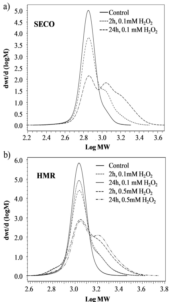
Fig. 5. Molar mass increase after VP treatment in the presence of 0.1 mM Mn^{2+} of: (a) SECO and (b) HMR. Controls correspond to VP-untreated SECO or HMR with 0.1 mM H_2O_2 at 24 h of incubation. Controls corresponding to VP-untreated HMR with 0.5 mM H_2O_2 were similar to the previous control and are not represented in (b).
