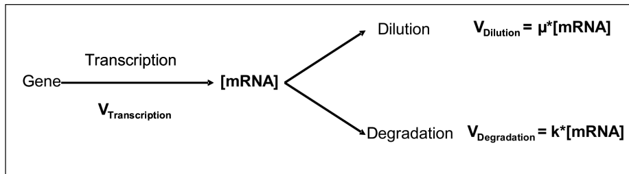
Figure 1. Cellular processes influencing mRNA concentration. Transcription, mRNA decay and dilution due to growth are involved. Dilution and degradation rates can be modeled as \mu * [\text{mRNA}] and k * [\text{mRNA}] , respectively, where \mu is the growth rate and k the degradation rate constant. doi:10.1371/journal.pone.0059059.g001
