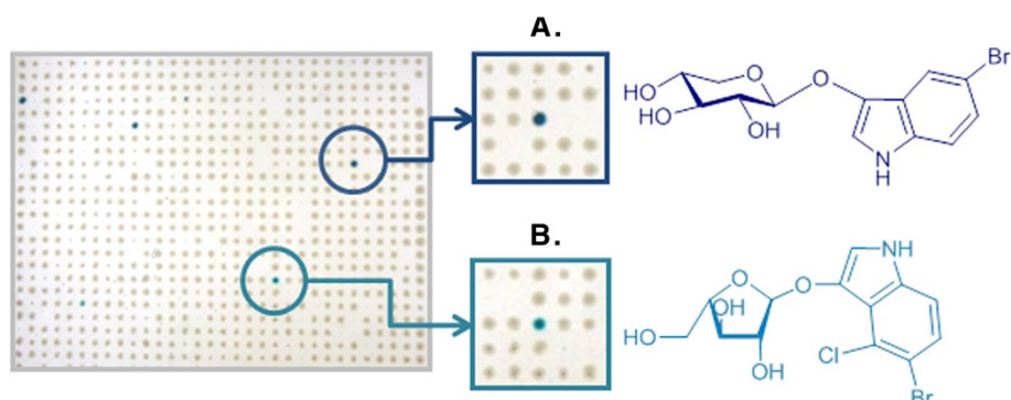
Figure 1 In vivo functional screening of metagenomic clones arabinofuranosidase. A. and B. xylosidase activities using the chromogenic substrates BI-Xylp and BCI-Araf respectively.
