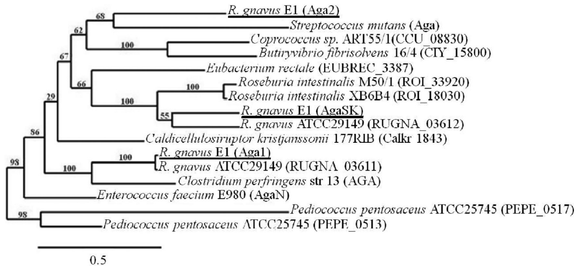
FIG 2 Unrooted phylogenetic tree of GH36 \alpha -galactosidases from Firmicutes . R. gnavus E1 \alpha -galactosidases Aga1, Aga2, and AgaSK are underlined. Percent bootstrap values are indicated. str, strain.
