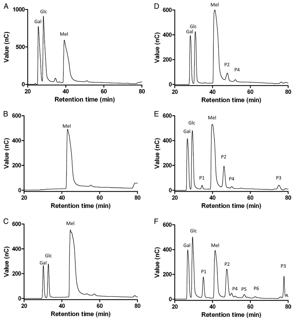
FIG 7 HPAEC-PAD analysis of self-condensation products of melibiose (2 M) incubated with Aga1 (15.7 nM). (A) Standards Glc, Gal, and Mel at 500 \mu M; (B) no-enzyme control after 150 h; (C) reaction after 1 h; (D) reaction after 10 h; (E) reaction after 24 h; (F) reaction after 150 h.
