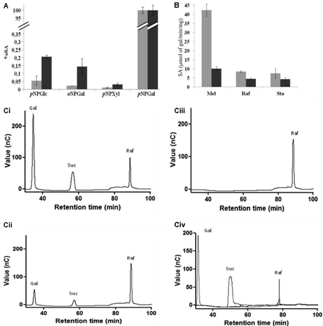
FIG 5 Substrate specificities of R. gnavus E1 Aga1 and Aga2. (A) Hydrolysis of pNP -pyranosides by R. gnavus E1 Aga1 (light gray) and Aga2 (dark gray). The recombinant enzymes were incubated with different sugars linked to pNP , and the cleavage of the linkage was estimated as the amount of pNP released in the reaction mixture. (B) Hydrolysis of natural substrates by R. gnavus E1 Aga1 (light gray) and Aga2 (dark gray). The specific activity was determined by quantifying the amounts of Gal released during incubation with the recombinant enzymes. (C) HPAEC-PAD analysis of hydrolysis products of Raf (12 mM) incubated for 4 h with Aga1 (114 nM; panel Ci) or Aga2 (234 nM; panel Cii) or a no-enzyme control (panel Ciii). All samples were diluted 1/10 prior to injection. Panel Cii shows an overlay of 0.5 mM standards of Raf (solid line), Suc (dashed line), and Gal (dotted line). nC, nanocoloumbs.
