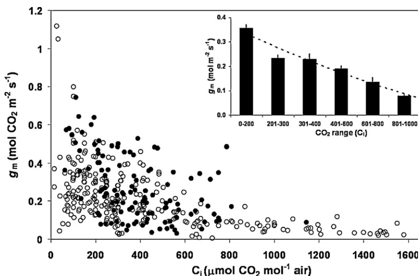
Fig. 5. Increasing CO_2 concentration reduces mesophyll conductance. g_m correlates with C_i over a broad range of ambient CO_2 concentrations and across a number of different species and growth forms. The isotopic method ( \delta^{13}C ) and the combined chl fluorescence and infrared gas exchange analysis method are shown in closed and open circles, respectively.
