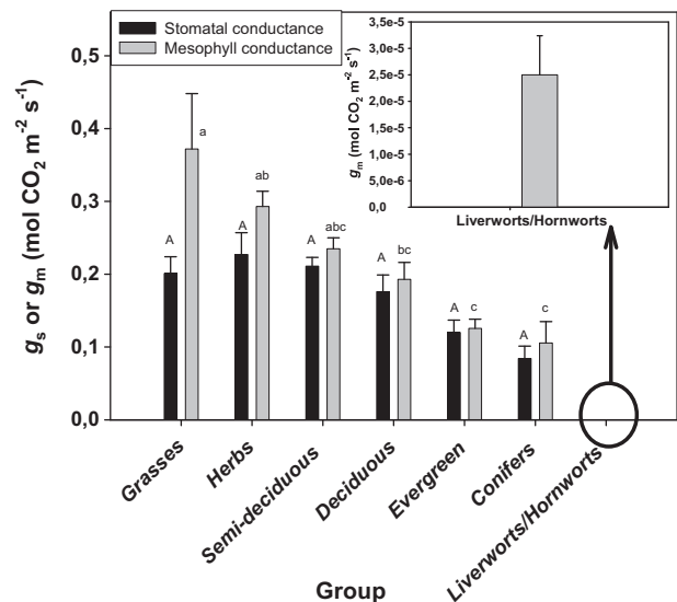
Fig. 1. Mesophyll conductance is greatest the more a species is phylogenetically evolved. Average \pm S.E. values for g_s and g_m in different pooled groups of plants. Data from liverworts and hornworts from [17], data for all other groups from [14]. Only data at light saturation and ambient temperature were considered. Capital letters indicate differences between means for g_s and lower case letters for g_m (Tuckey test, p < 0.05 , n = 3, 21, 2, 11, 25 and 6 for grasses, herbs, semi-deciduous, deciduous, evergreen and conifer species, respectively).
