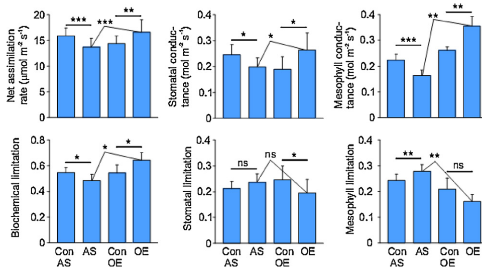
Fig. 3. Altered expression of aquaporins in relation to mesophyll conductance limitations of photosynthesis. Average (error bars show + S.E.) net assimilation rate, stomatal conductance to \text{CO}_2 and mesophyll diffusion conductance (upper panels) and relative photosynthetic limitation due to limited biochemical capacity, stomatal conductance and mesophyll diffusion conductance (lower panels) in transformed plants with reduced (AS, RNA-interference) and over-expressed (OE) aquaporins and corresponding controls (either wild type or plants transformed with the same construct used for AS and OE, but lacking the modified aquaporin expression phenotype). As the data represent one-to-one correspondence between data pairs (control vs. AS and control vs. OE and AS vs. OE within the given study), the averages between the treatments and corresponding controls and between AS and OE were compared by paired t -tests that is a more powerful statistical test than standard ANOVA [138]. Statistical significance as: ns, not significant; * P < 0.05 , ** P < 0.01 , *** P < 0.001 . The data are for Arabidopsis thaliana aquaporins atp1p1;2-1 and atp2p2;3-1 [32], Nicotiana tabacum aquaporin NtAQP1 [33–35] and Hordeum vulgare aquaporin HvPIP2;1 [36]. The data correspond to saturating light, leaf temperature of 25 °C and chamber \text{CO}_2 concentration of 280–400 \mu\text{mol mol}^{-1} . The relative limitations of photosynthesis were calculated according to [42] and the three limitations sum up to 1. Maximum carboxylase activity of Rubisco, V_{\text{cmax}} , needed for these calculations was determined by inverse modeling as in [43]. Means between treatment and corresponding controls and between AS and OE were compared by paired t -tests (ns, not significant; * P < 0.05 , ** P < 0.01 , *** P < 0.001 ).
