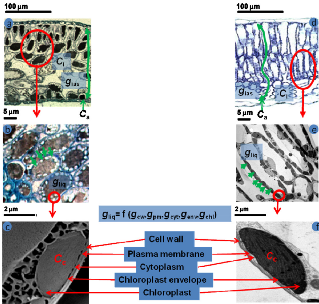
Fig. 2. Mesophyll conductance reflects the \text{CO}_2 diffusion pathway, which is composed of air, water and lipid barriers. Comparison of \text{CO}_2 diffusion pathway within the fully expanded needle of evergreen conifer Abies alba (a–c) and within the leaf of broad-leaved deciduous Populus tremula (d–f) according to light (a, b, d), scanning (c) and transmission electron (e, f) micrographs. Leaf cross-sections (a, d) illustrate the \text{CO}_2 gas phase diffusion pathway from ambient air ( C_a ) to sub-stomatal cavities ( C_i ) and from sub-stomatal cavities to outer surface of cell walls, C_{i,w} . The \text{CO}_2 concentration drawdown, C_a - C_i , depends on stomatal conductance, while the drawdown C_i - C_{i,w} is characterized by internal gas-phase diffusion conductance ( g_{ias} ) that is determined by effective mesophyll thickness and porosity. The micrographs of palisade tissue (b, e) demonstrate parallel diffusion pathways within cells (indicated with arrows for representative cells) that is determined by the exposure of chloroplasts to intercellular airspace. The representative micrographs of palisade cells (c, f) illustrate \text{CO}_2 diffusion pathways in liquid phase from mesophyll cell outer surface to chloroplasts. The \text{CO}_2 drawdown from outer surface of cell walls to chloroplasts ( C_c , C_{i,w} - C_c ) is determined by liquid-phase diffusion conductance g_{liq} that consists of cell wall (cw), plasma membrane (pm, not visible in the micrographs), cytoplasm (cyt), chloroplast envelope (env, not visible in the micrographs), and chloroplast stroma (chl). Micrographs from Peguero-Pina et al. [60] (a–c) and Tosens et al. [15] (d–f), with permission.
