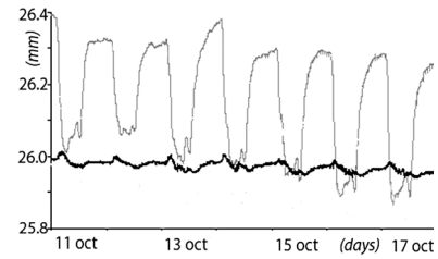
Figure 2. Extensometer variations recorded in 1999 during a quiet period. Grey values represent the raw data; black values are corrected.
