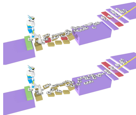
Fig. 12. HRP-2 in the re-planning scenario. After the red step stones are removed, a new sequence of contacts is re-planned. Hand contacts are not presented here for readability.
