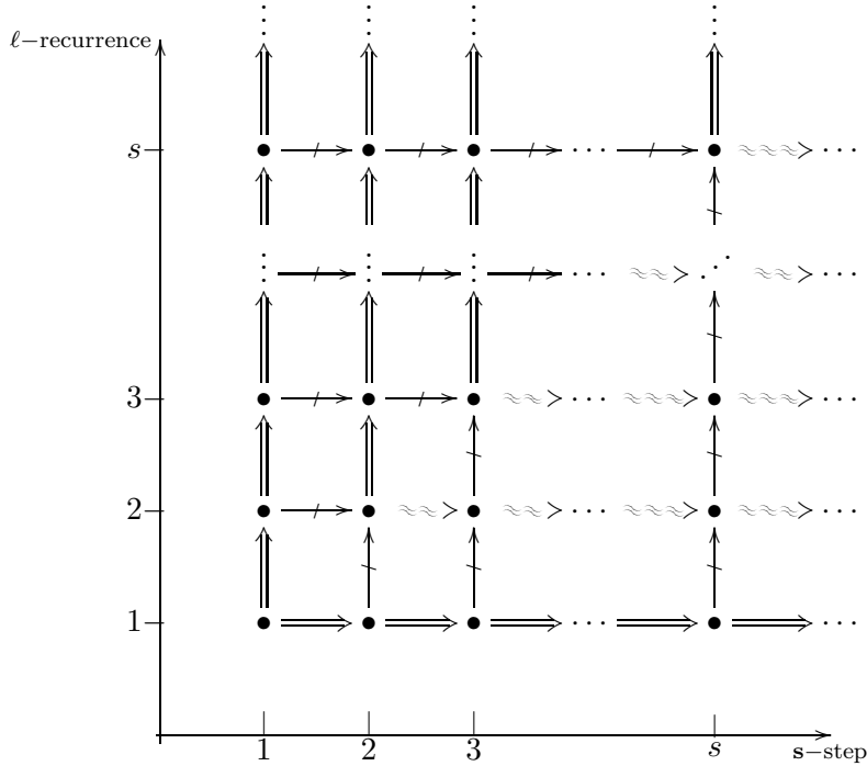
FIGURE 1. The horizontal axis represents the step of the nilsystem and the vertical axis represents the level of recurrence. The vertical implications are proven in Corollary 5.3 and counterexamples for vertical implications (with step greater than recurrence) are given by Example 5.11. Horizontal squiggly implications are proven only for affine nilsystems in Theorem 5.13, while the full horizontal implications are proven in Theorem 4.1. Counterexamples for the horizontal implications (with recurrence greater than step) follow from Corollary 5.3 and Corollary 5.10.
