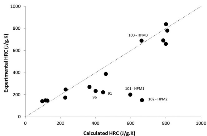
Fig. 14. Experimental versus calculated HRC for 16 phosphonate-based polymers.
