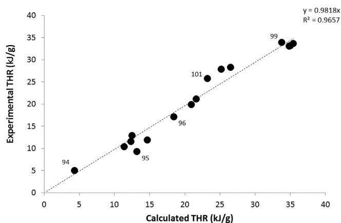
Fig. 13. Experimental versus calculated THR for 16 phosphonate-based polymers (labels correspond to polymers numbered in Table 1).
