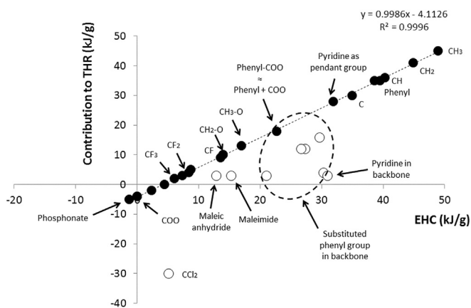
Fig. 8. Contribution to THR versus EHC calculated from the Huggett relation.
