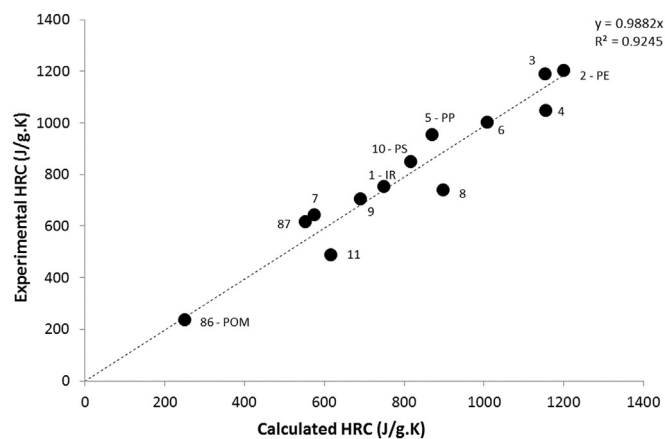
Fig. 2. Experimental versus calculated HRC for a first series of polymers (labels correspond to polymers numbered in Table 1).
