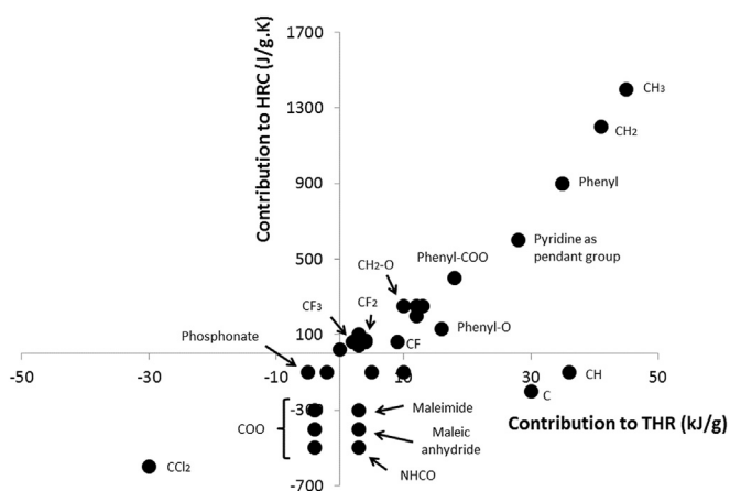
Fig. 9. Contribution to HRC versus contribution to THR for 31 groups.
