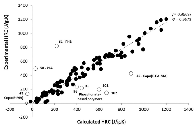
Fig. 7. Experimental versus calculated HRC for 107 polymers studied in this work (dashed line was plotted considering only black points – white points correspond to exceptions discussed later).
