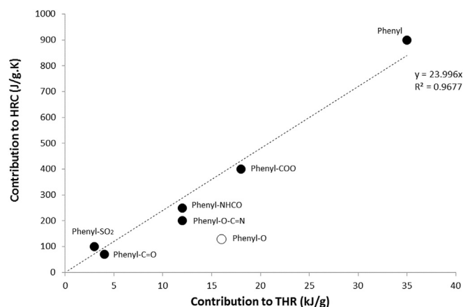
Fig. 10. Contribution to HRC versus contribution to THR for phenyl groups in backbone.
