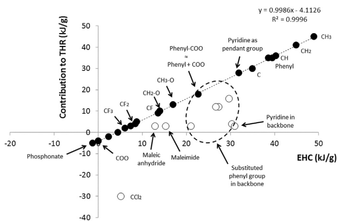
Fig. 8. Contribution to THR versus EHC calculated from the Huggett relation.
