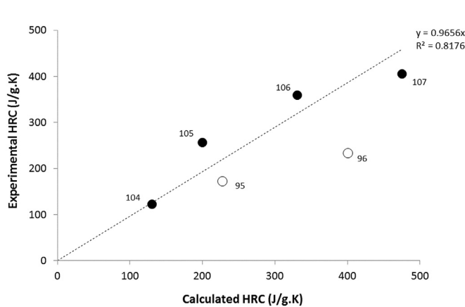
Fig. 5. Experimental versus calculated HRC for polymers containing a maleimide group (labels correspond to polymers numbered in Table 1).
