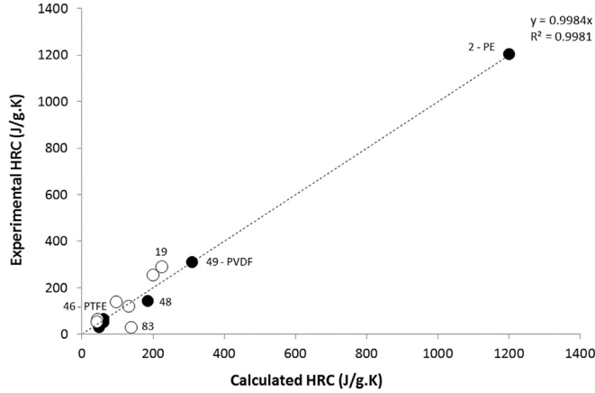
Fig. 3. Experimental versus calculated HRC for fluorinated polymers (labels correspond to polymers numbered in Table 1).
