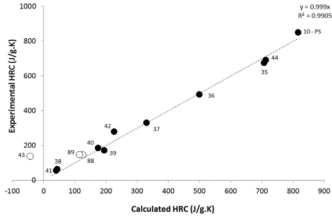
Fig. 4. Experimental versus calculated HRC for polymers containing a maleic anhydride group (labels correspond to polymers numbered in Table 1).
