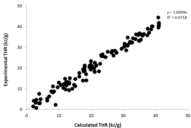
Fig. 6. Experimental versus calculated THR for 107 polymers studied in this work (using first database).
