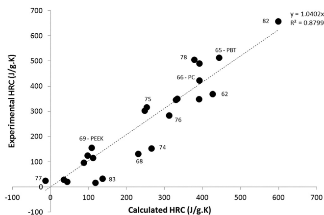
Fig. 11. Experimental versus calculated HRC for polymers containing various phenyl groups in the main chain (labels correspond to polymers numbered in Table 1).
