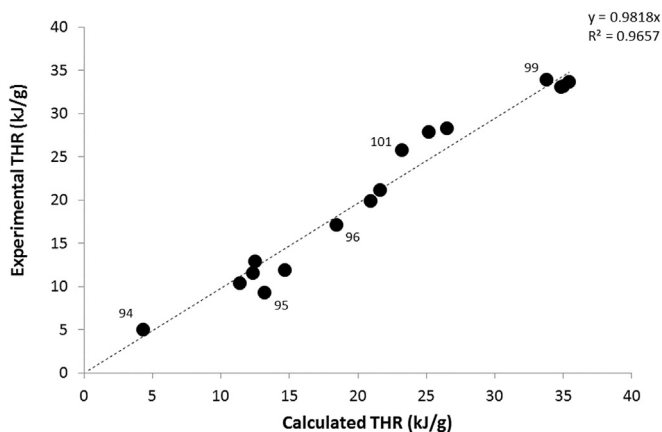
Fig. 13. Experimental versus calculated THR for 16 phosphonate-based polymers (labels correspond to polymers numbered in Table 1).
