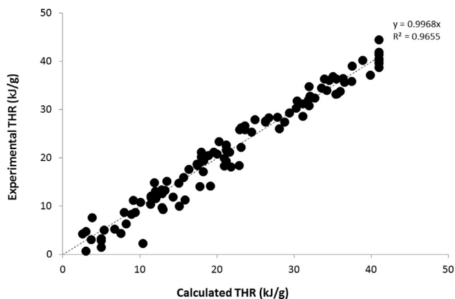
Fig. 15. Experimental versus calculated THR of 107 polymers according to the second database.
