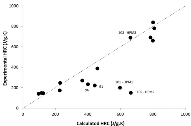
Fig. 14. Experimental versus calculated HRC for 16 phosphonate-based polymers.
