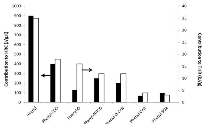
Fig. 12. —Contributions to THR and HRC for various substituted phenyl groups in the polymer main chain.
