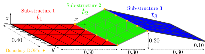
Figure 1: Plate structure composed of 3 flat sub-structures with their own thicknesses
