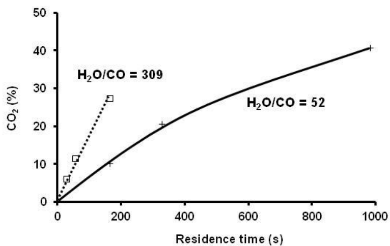
Fig.3: Transformation of CO alone into CO 2 versus the residence time of CO. Effect of the H 2 O/CO ratio. (T = 523°K, P = 2 MPa, CoMoS/Al 2 O 3 )
