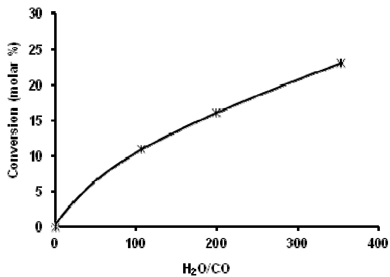
Fig.5: Transformation of the model feed: Effect of the H 2 O/CO ratio on the transformation of CO into CO 2 . (T = 523°K, P = 2 MPa, P CO = 1.31 kPa, CoMoS/Al 2 O 3 , residence time = 3s, H 2 /feed = 360NL/l)
