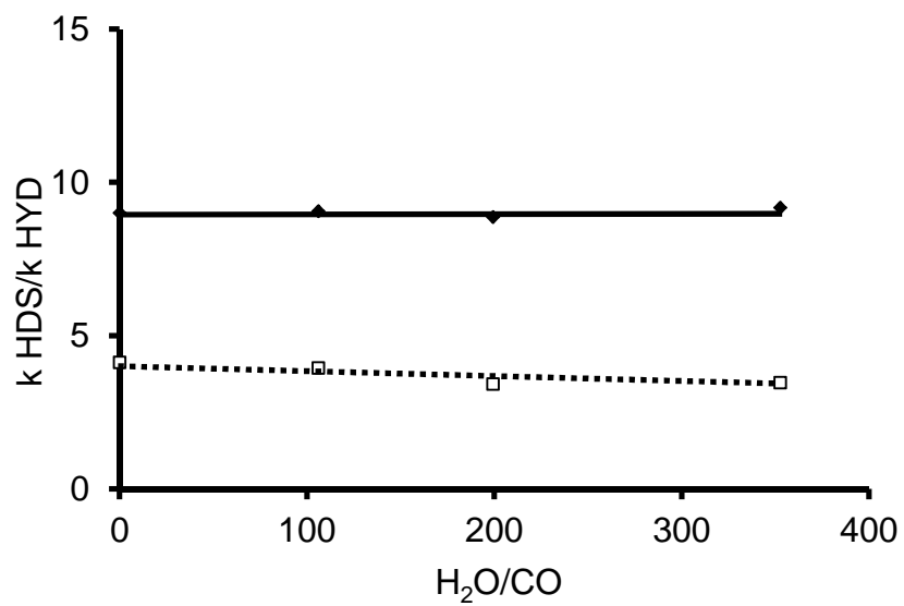
Fig.6: Transformation of a model FCC gasoline. Effect of different H 2 O/CO molar ratio and initial conversion of 2MT (C 0 , 2MT) on the k HDS /k HYD ratio (C 0 ,2MT = 18,9%:□, C 0 ,2MT = 41% ◆(T = 523°K , P = 2MPa, H 2 /feed = 360 NL/L, CoMo/Al 2 O 3 ).
