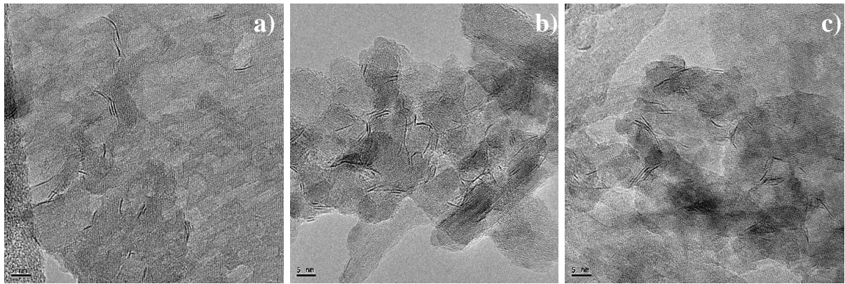
Fig.8: TEM analysis of CoMoS/Al 2 O 3 a) freshly sulfided b) after the transformation of the model feed c) after the transformation of the model feed in the presence de 462 kPa of water (scale : 5 nm)
