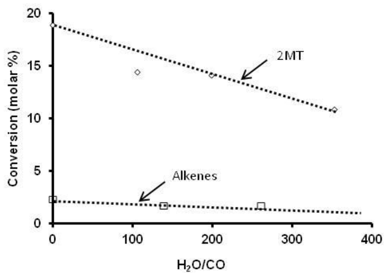
Fig.4: Transformation of the model feed: Effect of the H 2 O/CO ratio a) 2MT conversion, b) alkenes conversion. (T = 523°K, P = 2 MPa, P CO = 1.31 kPa, CoMoS/Al 2 O 3 , residence time = 3s, H 2 /feed = 360NL/l)
