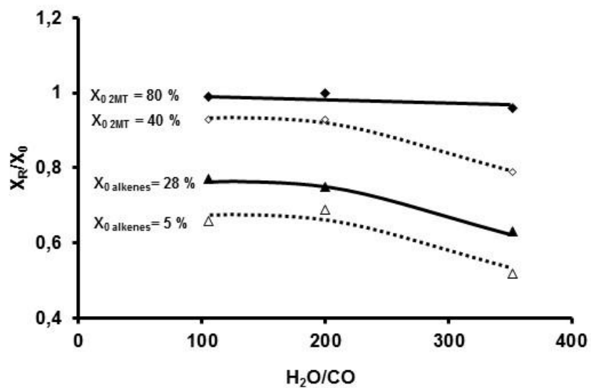
Fig. 7: X_{Rr}/X_0 ratio ( X_R : conversion measured after stopped water, X_0 : initial conversion as a function of H_2O/CO ratio on the transformation of 2MT and alkenes (23DMB2N+23DMB1N) in mixture ( T = 523^\circ K , P = 2 MPa, P_{CO} = 1,31 kPa, CoMo/ Al_2O_3 , H_2/feed = 360 NL/L)
