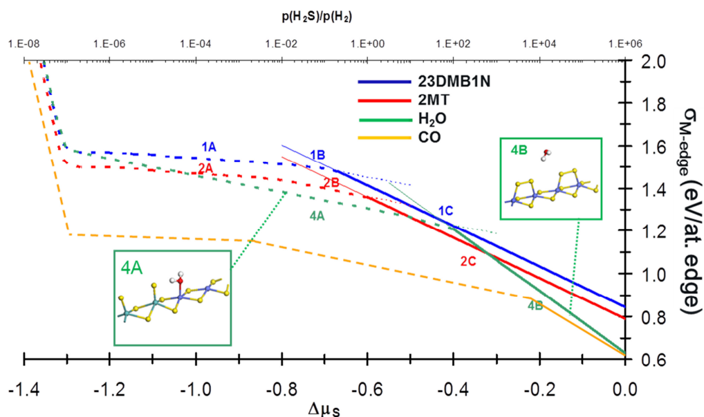
Fig. 11: Evolution of the edge energy as a function of the sulfur chemical potential ( \Delta\mu_s ) for the 4 relevant molecules adsorbed on CoMoS M-edge. Partial pressures and temperature are chosen in agreement with experimental conditions: P(23\text{DBM1N}) = 150 kPa, P(2\text{MT}) = 3 kPa, P(\text{H}_2\text{O}) = 15 kPa, P(\text{CO}) = 1.31 kPa. The p(\text{H}_2\text{S})/p(\text{H}_2) axis is determined for T = 525 K. Dashed lines correspond to the partially promoted M-edge ( \text{Co}/\text{Mo} = 0.5 ), full lines to the fully promoted one. Structure 4A (resp. 4B) corresponds to water adsorbed on the partial Co promotion with 25.0% of sulfur (resp. on the fully promoted edge with a S content of 50%). The description of structures 1A-1C and 2A-2C is given in Ref. [27]. Energetic data for CO are taken from [15].
