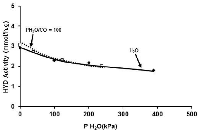
Fig 15 Transformation of alkenes alone. Comparison of the effect of CO and water. (T = 523°K, P = 2 MPa, CoMo/Al 2 O 3 , H 2 /charge = 360 NL/L)
