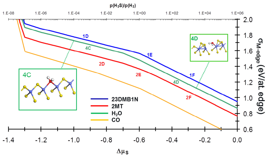
Fig.12: Evolution of the edge energy as a function of the sulfur chemical potential ( \Delta\mu_S ) for the 4 relevant molecules adsorbed on CoMoS S-edge for the same conditions as in Fig. 8. Structure 4C (resp. 4D) correspond to water adsorbed on the fully promoted S-edge with a S content of 37.5% (resp. 62.5%). Structures 1D-1F and 2D-2F are given in Ref. [27]. Energetic data for CO are taken from [15].
