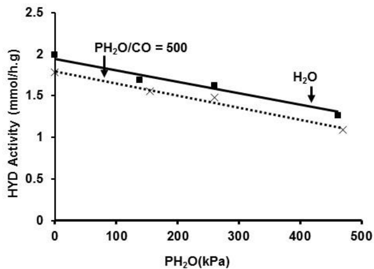
Fig 17: Transformation of the model feed. HYD activity – alkenes transformation. Comparison of the effect of CO and water. (T = 523°K, P = 2 MPa, CoMo/Al 2 O 3 , H 2 /charge = 360 NL/L)
