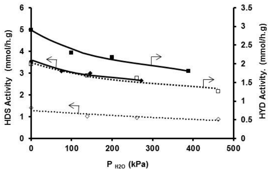
Fig. 1: Impact of the water partial pressure in the HDS (2MT) and HYD (alkenes) activities. 2MT ( \blacklozenge , full line) and 23DMB2N ( \blacksquare , full line) transformation alone and with 2MT ( \diamond , dotted line) and 23DMB2N ( \square , dotted line) transformation in mixture. ( T = 523K , P = 2 \text{ MPa} , ratio H_2/\text{feed} = 360 \text{ NL/L} , \text{CoMoS}/\text{Al}_2\text{O}_3 ).
