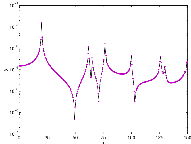
Figure 8: FRF of the stiffened cylindrical shell: FE solution (—) and WFE solution when the central periodic structure is modeled by means of m = 125 wave modes (•••).
