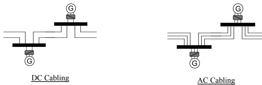
Figure 2.4: Interconnecting cables routes for AC and DC technology
