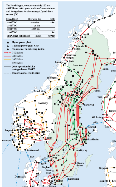
Figure 2.48: Electric power transmission grid in Sweden [105]
