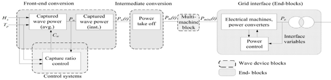
Figure 3.32: Outline of ocean wave energy converter model
