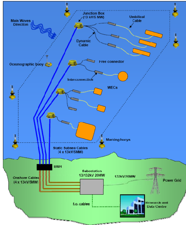
Figure 3.1: bimep architecture.
