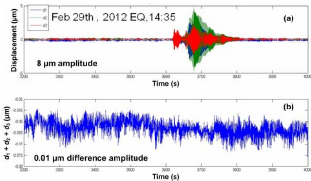
Fig. 8. (a) IF-LINES response (DC – 10 Hz) to M6.5 Japan Earthquake at end Feb 2012 with max. amplitude of ~8 μm detected; (b) Tri-axial redundancy validates instrument's capacity for common-mode compensation
