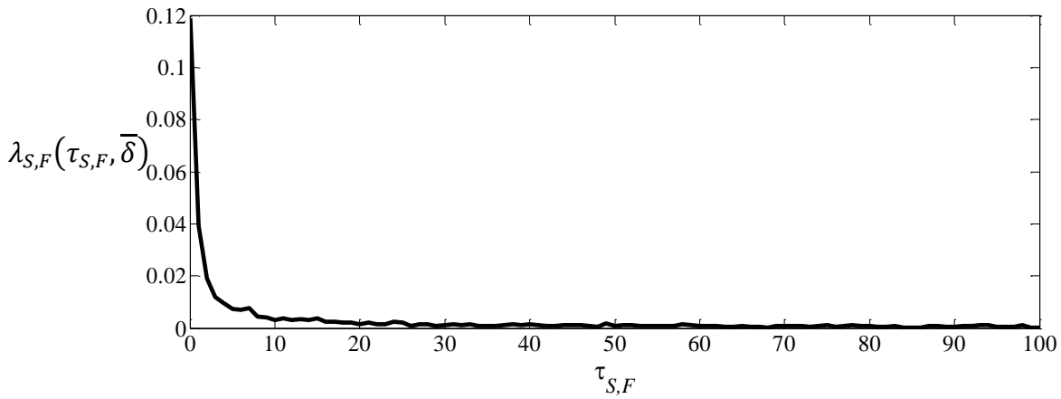
Fig. 8 Transition rate between states S and F
