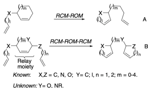
Scheme 1. Some synthetically useful metathetic cascades.
