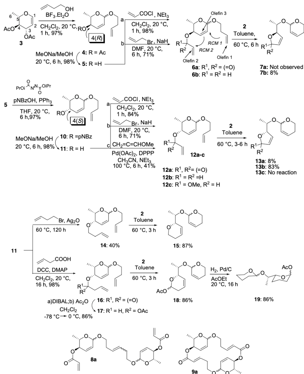
Scheme 2. RCM-ROM-RCM of 3,6-dialkoxy-3,6-dihydro-2H-pyrans.
