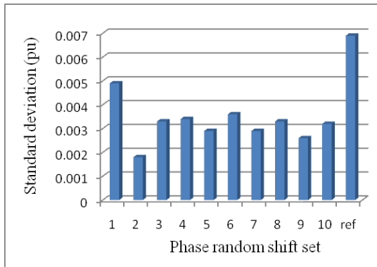
Figure 8 Maximum voltage standard deviation
