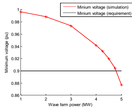
Figure 11 Minimum voltages
