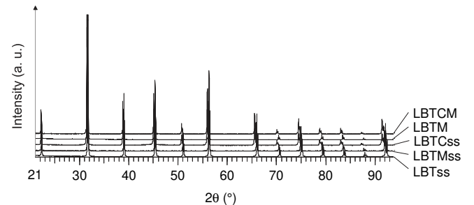
Fig. 2. XRD patterns of LBTss, LBTMss, LBTcSs, LBTM, and LBTcM after synthesis in air and reduction at 900 °C for 48 h in \text{Ar}/\text{H}_2(98/2) .
