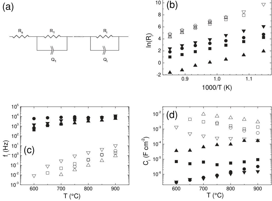
Fig. 8. Evolution with temperature of main characteristic electrochemical parameters for LBTss/BIT/YSZ/BIT/LBTss ( \Delta, \blacktriangle ), LBTcSSs/BIT/YSZ/BIT/LBTcSSs ( \square, \blacksquare ), LBTmSSs/BIT/YSZ/BIT/LBTmSSs ( \circ, \bullet ), and LBTcM/BIT/YSZ/BIT/LBTcM ( \nabla, \blacktriangledown ) symmetrical cells studied in \text{H}_2/\text{H}_2\text{O}(97/3) . (b) Specific resistances R_i (Arrhenius plot), (c) apex frequencies f_i , and (d) specific capacitances C_i . Closed and open symbols are for HF and LF contributions, respectively. In (a), the equivalent circuit scheme applied to fit impedance spectra ( i = 2 in our case).
