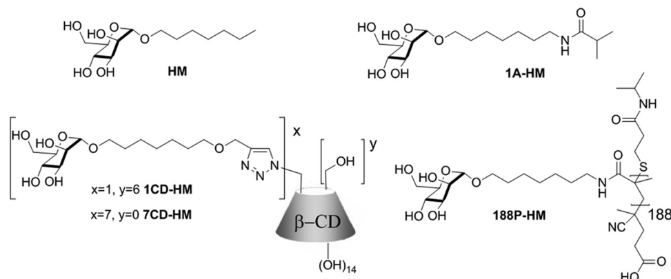
FIG 5 Structures of HM-based mannosides assessed for antiadhesive properties against the AIEC reference strain LF82. HM, 1A-HM (this study), 1CD-HM and 7CD-HM, and 188P-HM.
