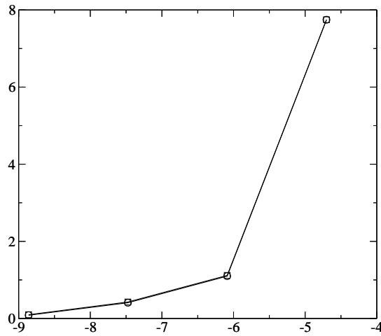
Figure 22: \rho v -error wrt. \log\left(\left(\frac{h_0}{2K}\right)^2\right) in the 2D pipe
