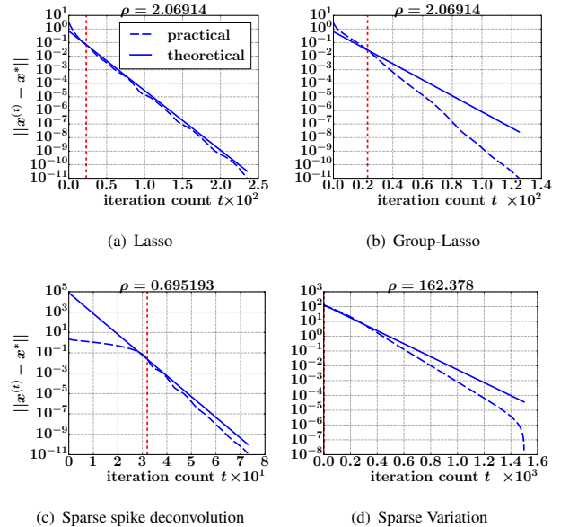
Fig. 2: Experimental results: Local Q-linear convergence for ADMM on problem (1). The “theoretical” line is the exponential curve t \mapsto \|x^{(0)} - x^*\| r(T'_\rho(x^*))^t . The red broken vertical line marks the instant \mathcal{A}_z(x^*) is identified. We can see from figure that the upper bound for the local convergence rate (Theorem 1) is satisfied. Each shown thumbnail is for the value of \rho for which the spectral radius r(T'_\rho(x^*)) was smallest.
