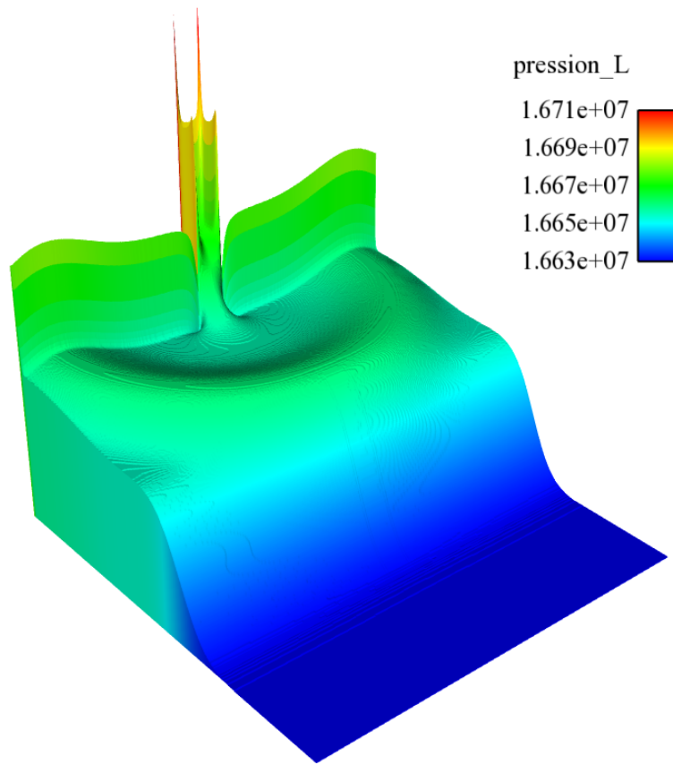
Figure 9: Heated wall: contours of the liquid pressure P_L in the computational domain at time T = T1 .
