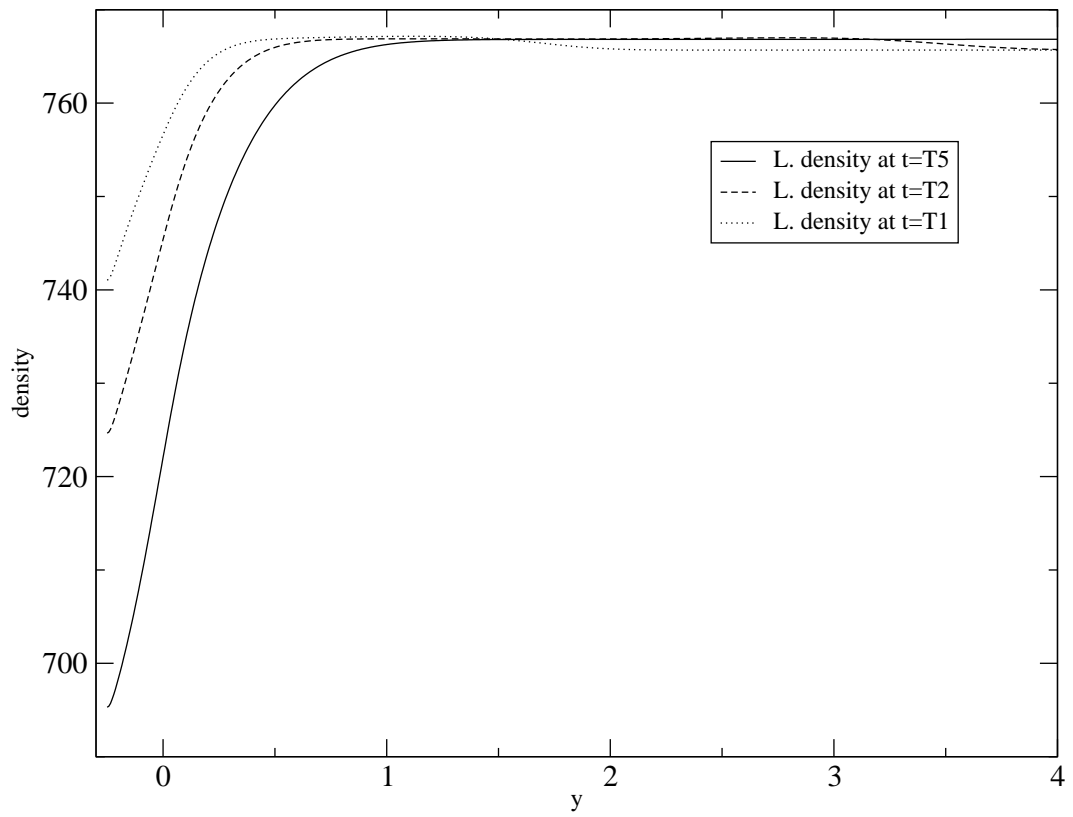
Figure 10: Heated wall: y -profile of the liquid density \rho_l at three distinct times T = T1 (dotted line), T2 (dashed line), T5 (plain line), at: x = 2 . The small cavity in the wall boundary corresponds to -0.25 < y < 0 .
