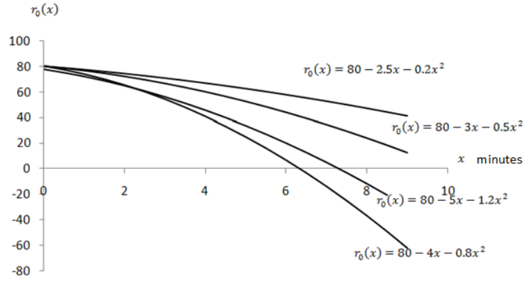
Figure 5: Remanufacturing cost-time
