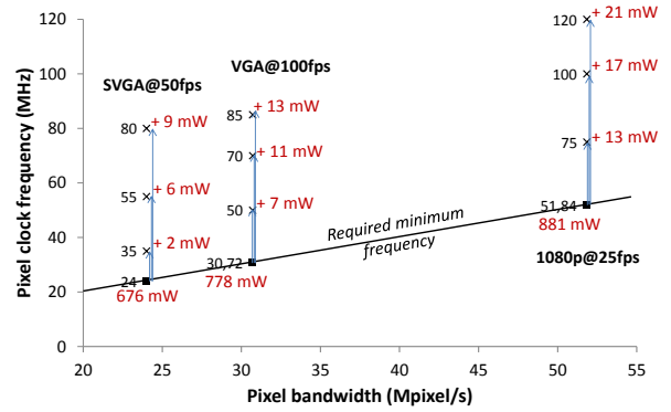
Fig. 7: Power savings by frequency tuning
